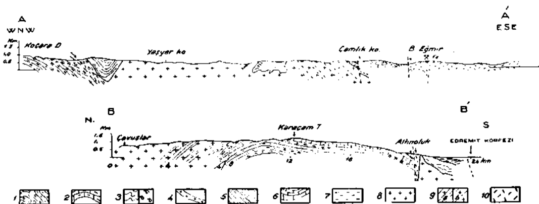
Fig. 2 - Sections AA' and BB' of Kazdağ region. (Compare Plate I)
