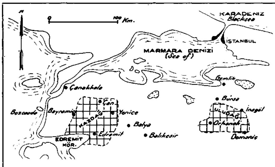
Fig. 1 - Location of investigated areas
