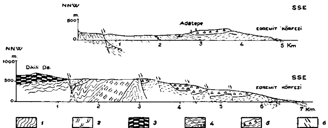
Fig. 4 • Sections west of Küçük Kuyu. (Compare Plate I)
